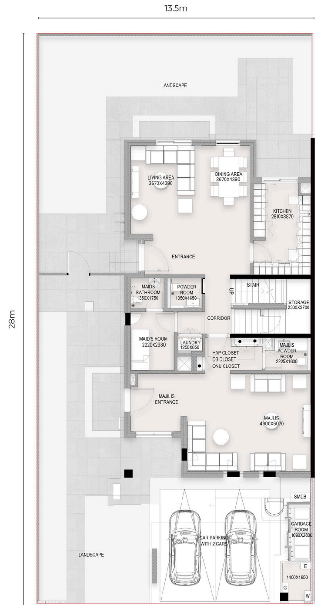
GROUND FLOOR
