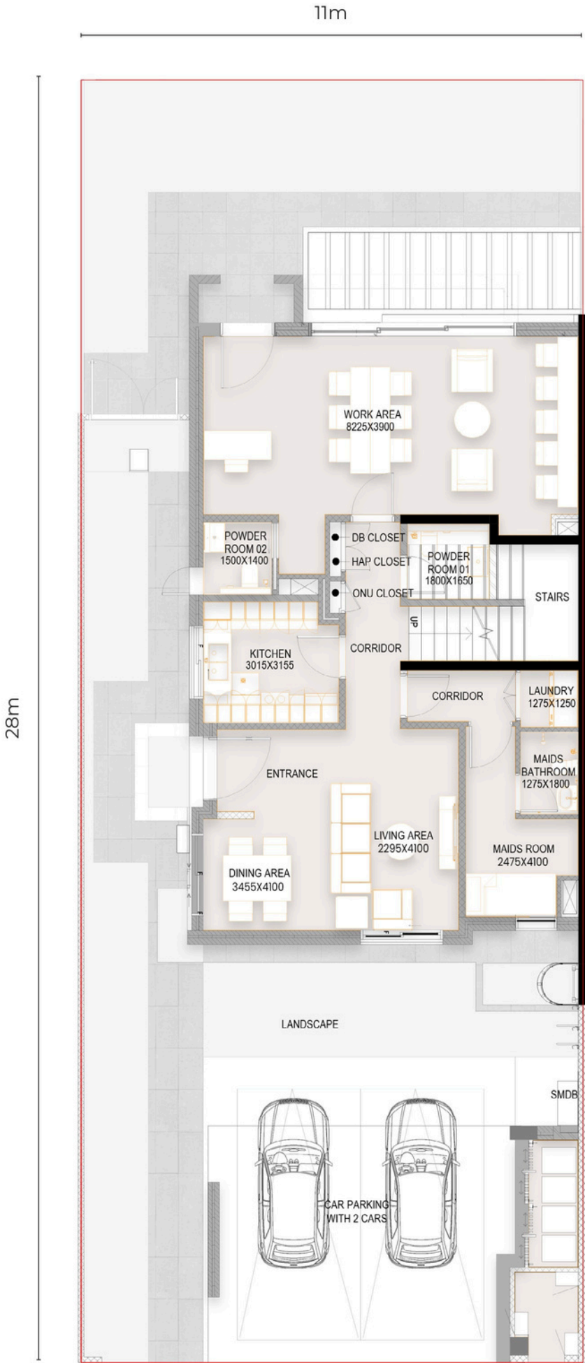
GROUND FLOOR
