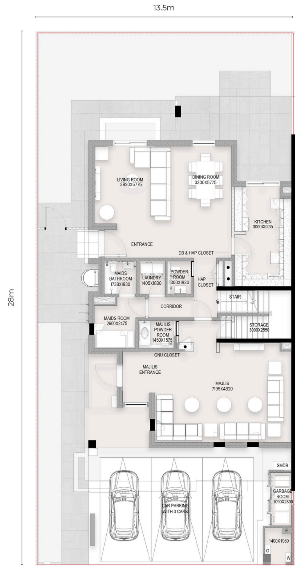
GROUND FLOOR
