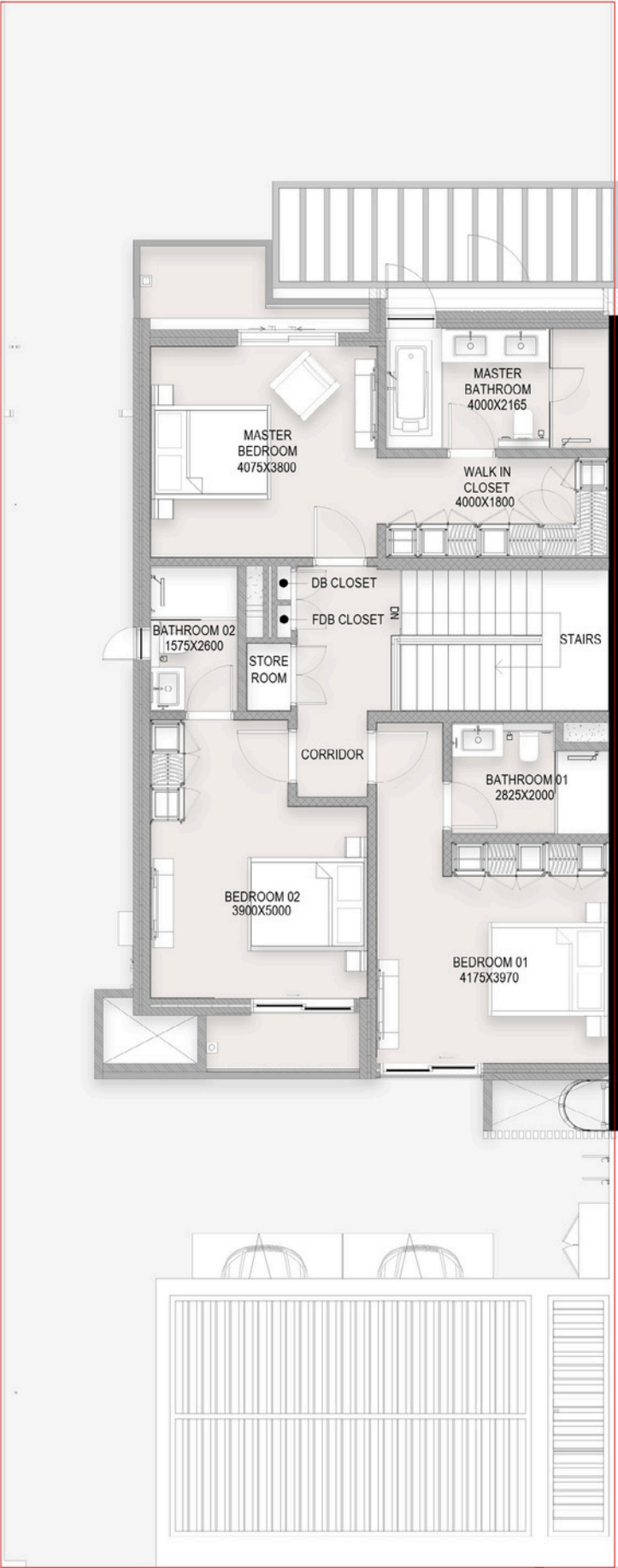
FIRST FLOOR
