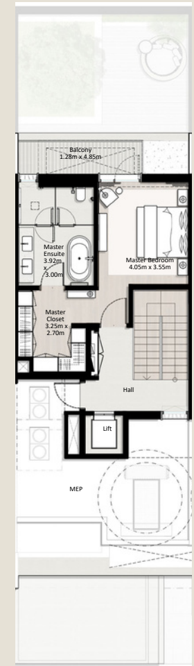
SECOND FLOOR
