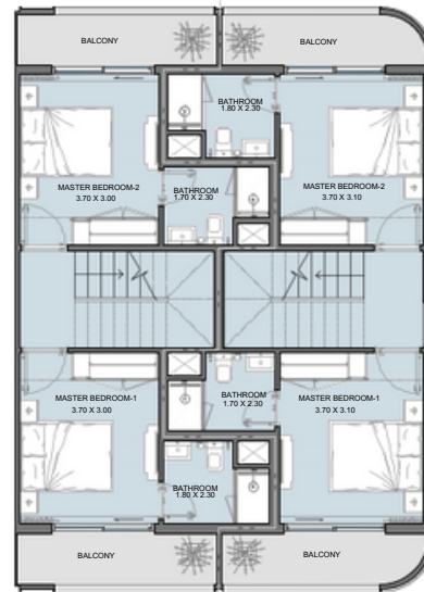
FIRST FLOOR Middle Unit
